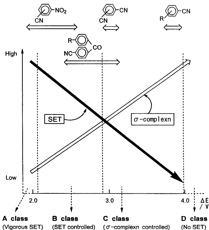
Figure 1. Illustration: relative degree of participation of efficiency of SET and \sigma -complexation for IDMg and Grignard reactions with monofunctional substrates. Given bifunctional compounds accompanied by short arrows indicate, for comparison, approximate \Delta E values for the present IDMg reactions
